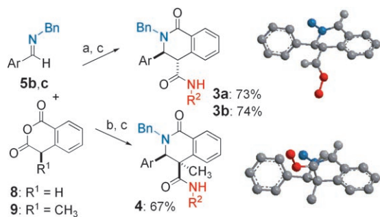
Scheme 3. Conditions: a) 5a or b + 8 , CH 2 Cl 2 , 23 °C; b) 5b or c + 9 , benzene, 23 °C, c) (p-CH 3 OC 6 H 5 )CH 2 CH 2 NH 2 , HATU. Minimized (MM2) structures of des-iodo- 3b and 5 , N-CH 3 groups depicted for clarity.
